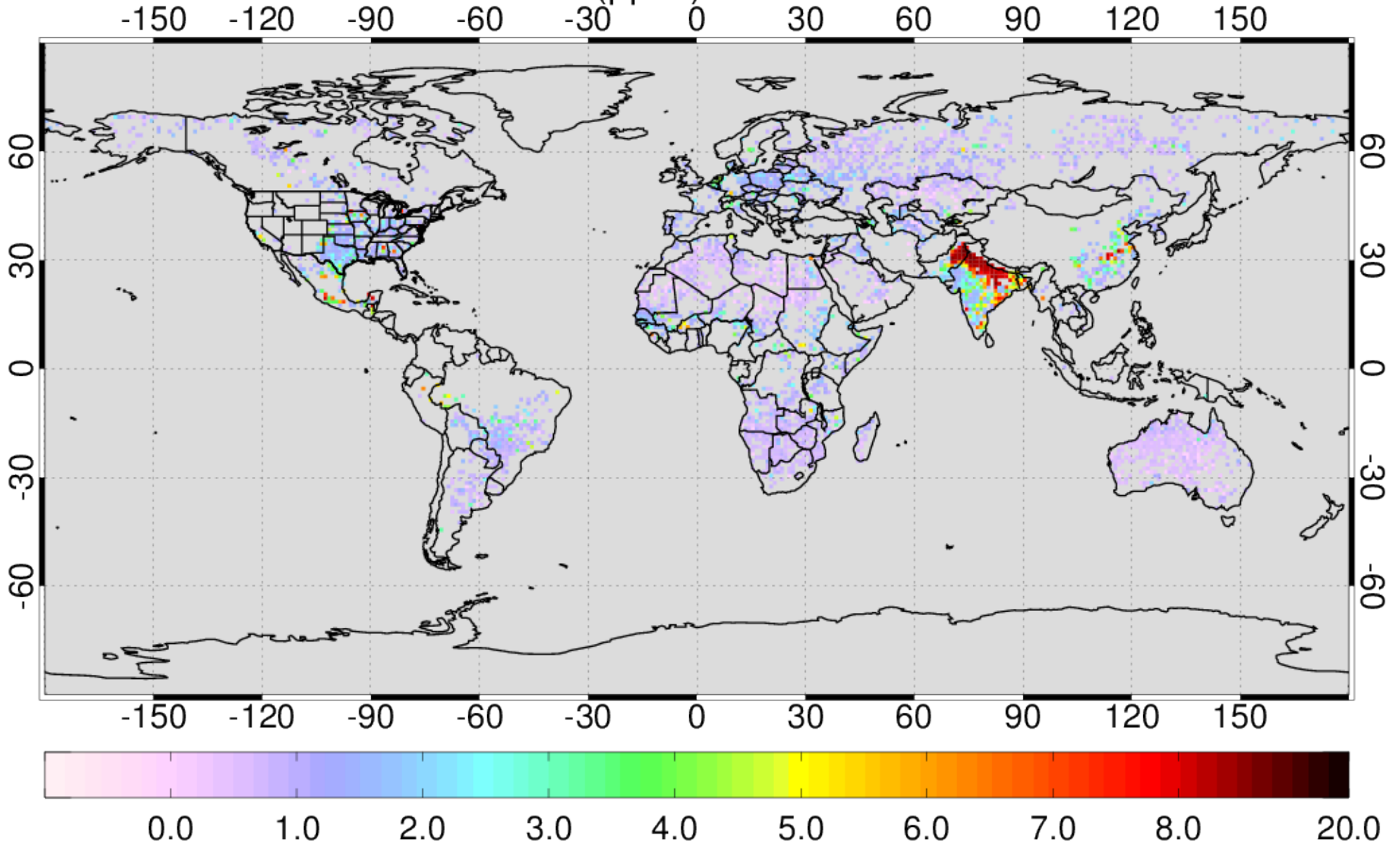
AIRS NH3 VMR (ppbv) at 840hPa for 201105
