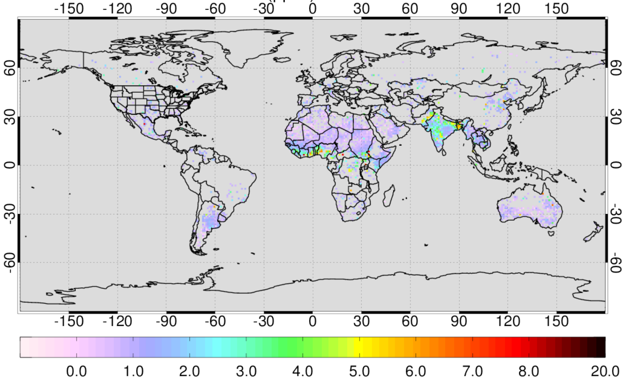
AIRS NH3 VMR (ppbv) at 840hPa for 201102
