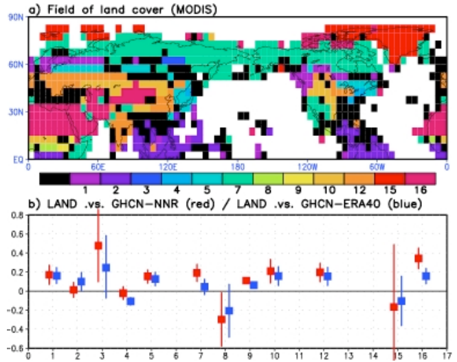
Fig. 2. (a) Land cover map derived from MODIS. Grid boxes in which the dominant land cover type covers less than 40% are colored black and not used in the analysis presented in panel (b). (b) the mean OMR trend of “GHCN-minus-NNR” (red), and “GHCN-minus-ERA40” (blue) per decade ( ^{\circ}\text{C}/\text{decade} ) over the NH as a function of land types. Filled squares represent the mean OMR trends and vertical lines the error bars at 95% significance level. The OMR trend per decade is obtained by taking the average of two decadal mean difference (90's - 80's and 70's - 60's).
