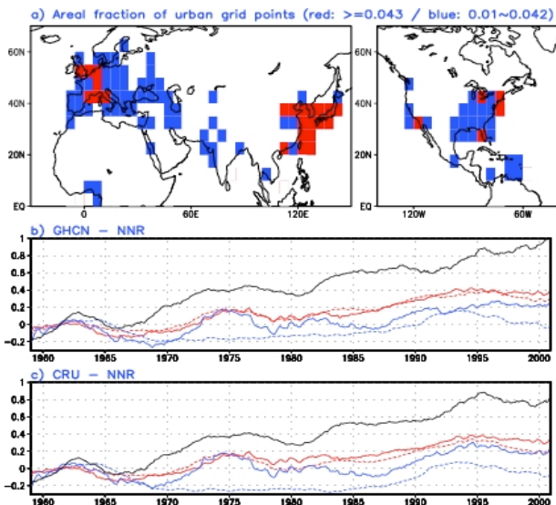
Fig. 3. a) Geographical distribution of urban grids ( 5^\circ \times 5^\circ ). Grid boxes where the fractional area of 1\text{km} \times 1\text{km} urban pixels is greater than 0.043 (in red), and between 0.01 and 0.042 (in blue) are categorized as big (small) urban areas. Time series ( ^\circ\text{C} ) of b) GHCN-NNR, and c) CRU-NNR, for the areas of big urban areas (red solid), small urban areas (red dashed), agriculture (blue solid), natural broadleaf (blue dashed), and barren areas (black solid), respectively.
