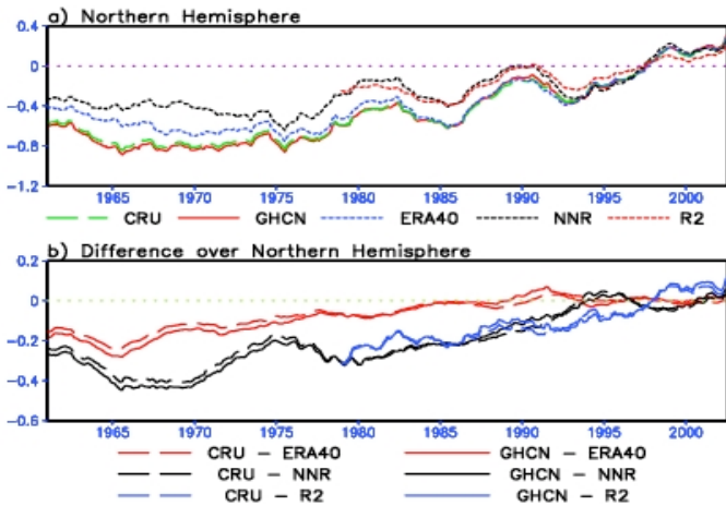
Fig. 1. Time series (three-year running mean) of (a) land surface temperature anomalies ( ^{\circ}\text{C} ) derived from CRU, GHCN, ERA40, NNR, and R2 and (b) the OMRs. Anomaly values are obtained by removing the 30-yr mean from 1961 to 1990 and they are further adjusted to have zero mean over the last 10 years (1993-2002).
