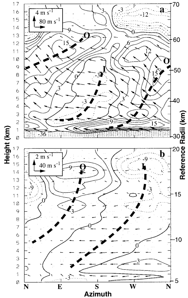
FIG. 3. The azimuth–height cross sections of the temporally averaged system-relative radial flow (every 3\text{ m s}^{-1} ) with the downdrafts shaded that are taken along the slanting surfaces (a) in the eyewall (i.e., from R = 30\text{ km} at the surface to R = 70\text{ km} at the 17-km height), and (b) in the eye (i.e., from R = 5\text{ km} at the surface to R = 20\text{ km} at the 17-km height) from the 56–57-h integration. The right axes show the radius in km at a few selected heights. Thick dashed lines denote the axes of incoming (I) and outgoing (O) air. Solid (dashed) lines are for positive (negative) values. In-plane flow vectors are superposed.
