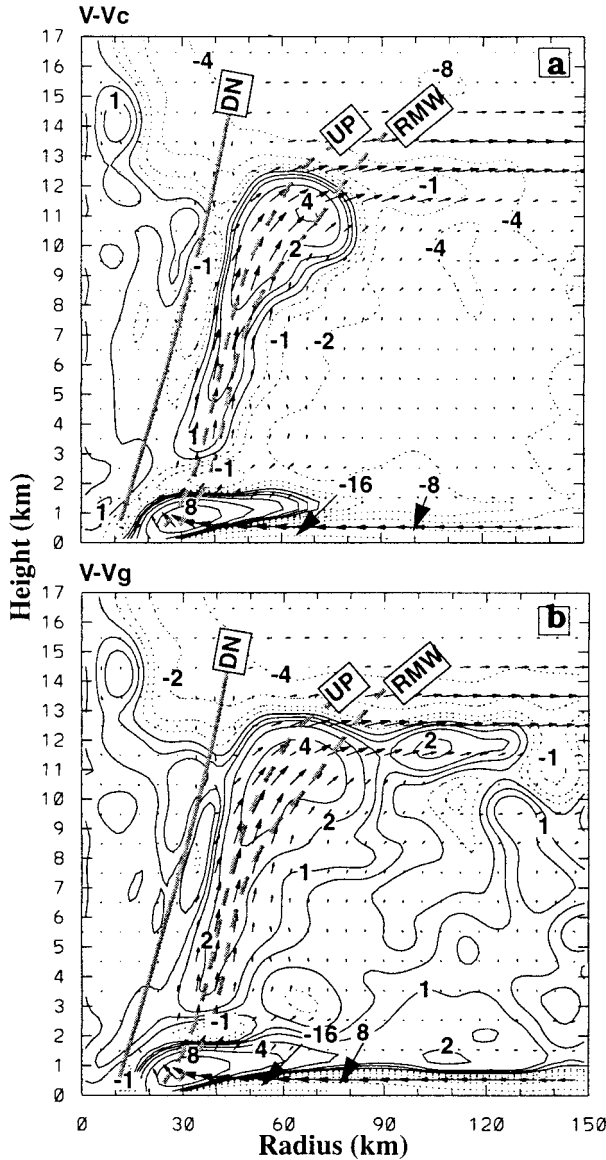
FIG. 7. As in Fig. 1 but for (a) acyclostrophic winds ( V - V_c ), and (b) agradiant winds ( V - V_g ), contoured at 0, \pm 0.5 , \pm 1 , \pm 2 , \pm 4 , \pm 8 , and \pm 16 \text{m s}^{-1} . In-plane full-flow vectors are superposed.
