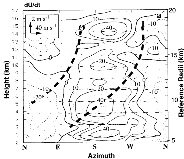
FIG. 11. As in Fig. 3b but for the Lagrangian radial momentum tendency ( dU/dt ) in the eye, contoured at 0, \pm 10 , \pm 20 , and \pm 40 \text{m s}^{-1} , with the inflow shaded.
