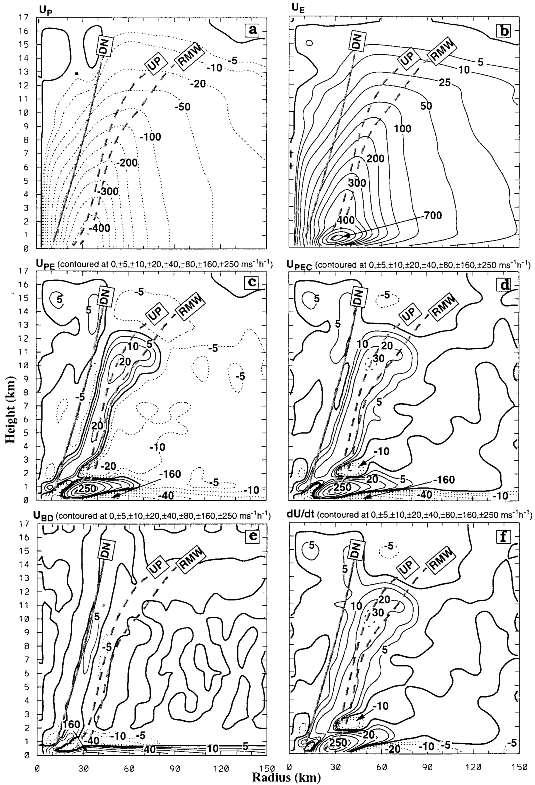
FIG. 6. As in Fig. 1 but for the radial momentum budget (unit: m\ s^{-1}\ h^{-1} ): (a) the radial pressure gradient force ( PGF_R = U_p ), (b) the centrifugal force ( U_E ), (c) the cyclostrophic force imbalance ( U_{PE} = U_p + U_E ), (d) the gradient force imbalance ( U_{PEC} = U_{PE} + U_C ), (e) the diffusion and boundary layer effects ( U_B ), and (f) the Lagrangian tendency ( dU/dt ).
