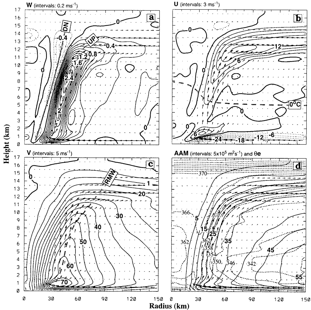
FIG. 1. Radius–height cross sections of the hourly and azimuthally averaged (a) vertical velocity ( W ) at intervals of 0.2 \text{ m s}^{-1} , (b) radial winds ( U ) at intervals of 3 \text{ m s}^{-1} , (c) tangential winds ( V ) at intervals of 5 \text{ m s}^{-1} , and (d) absolute angular momentum (AAM, solid) at intervals of 5 \times 10^5 \text{ m}^2 \text{ s}^{-1} and equivalent potential temperature ( \theta_e , dashed) at intervals of 4 \text{ K} , superposed with the cross-sectional flow vectors, taken from the 56–57-h integration or the period 2000–2100 UTC 23 Aug 1992. The radius of maximum wind, and the axes of the eyewall updrafts and the inner-edge downdrafts are represented by RMW, UP, and DN, respectively.
